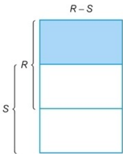
(e) Set difference
