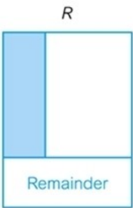
(h) Division (shaded area)
