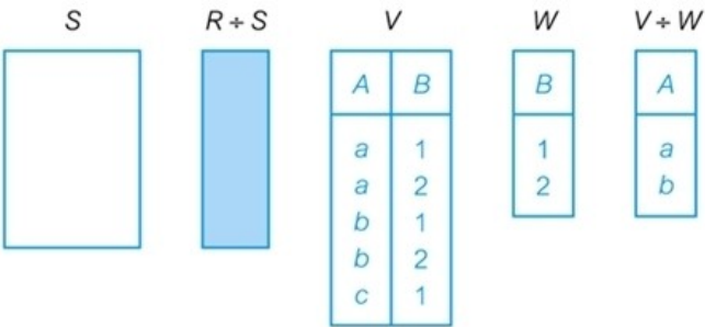
(h) Division (shaded area)
